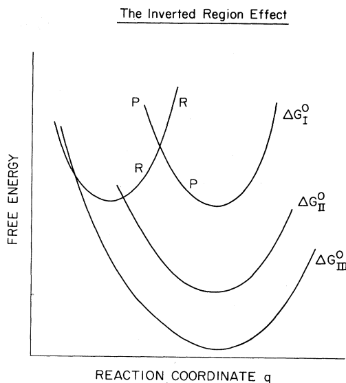
FIG. 6. Plot of the free energy G vs the reaction coordinate q , for reactants (R) and products (P), for three different values of \Delta G^0 , the cases I to III indicated in Fig. 7 (Marcus and Siddarth, Ref. 2).
