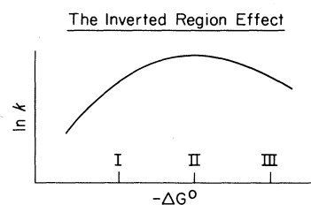
FIG. 7. Plot of \ln k , vs -\Delta G^0 . Points I and III are in the normal and inverted regions, respectively, while point II, where \ln k , is a maximum, occurs at -\Delta G^0 = \lambda (Marcus and Siddarth, Ref. 2).
