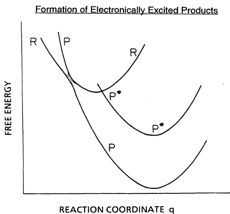
FIG. 9. A favored formation of an electronically excited state of the products (Marcus and Siddarth, Ref. 2).
