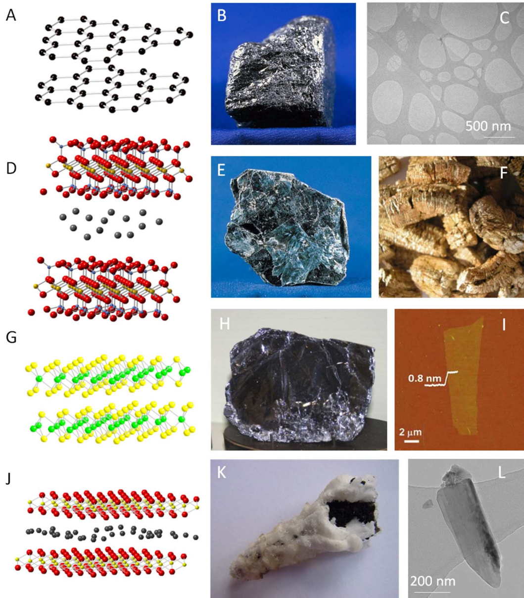
Fig. 1. Crystal structures, naturally occurring forms, and exfoliated products for four example layered materials. (A) Graphite consists of alternating stacks of hexagonally arranged carbon atoms (black spheres),
